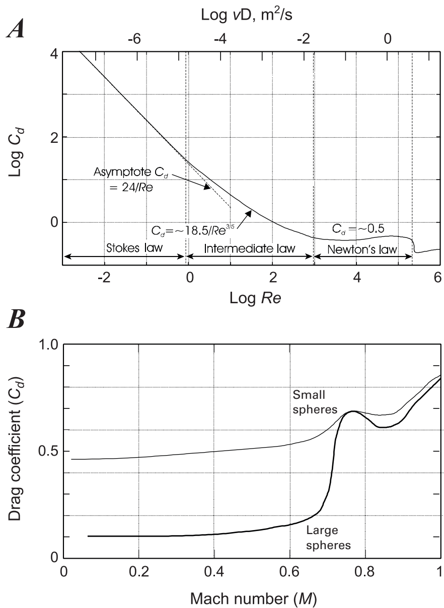
Figure 3. (A) Log drag coefficient ( C_d ) for spheres as a function of log Reynolds number, at low Mach number (from Bird and others, 1960, p. 192). Tick marks at top of plot give the product of velocity ( v ) times diameter ( D ) for spheres traveling in a fluid with the viscosity ( 1.8 \times 10^{-5} Pa s) and density ( 1.18 \text{ kg/m}^3 ) of air at 25^\circ \text{C} , 1 atm pressure. (B) Drag coefficient for spheres in air at varying Mach numbers (from Hoerner, 1965). Top curve represents drag coefficients for spheres at Reynolds numbers below the critical transition ( Re = \sim 2 \times 10^5 ) shown in figure 3A, whereas the lower curve represents drag coefficients for large spheres at Re above that transition.
