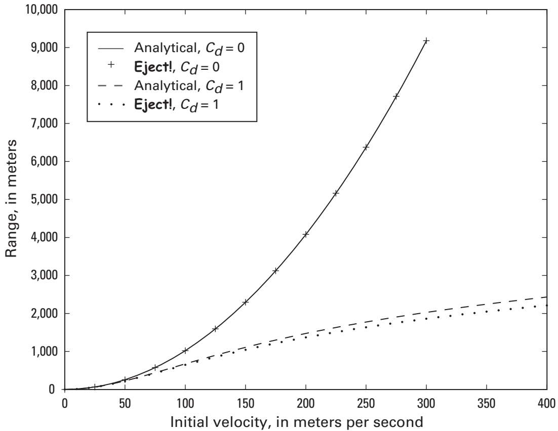
Figure 5. Range ( x_{final} ) versus initial velocity for a 40-centimeter diameter spherical block, with \rho_r = 2,500 \text{ kg/m}^3 and \theta = 45^\circ . Solid line gives the analytical solution for C_d = 0 ; crosses give the range calculated by Eject! for the same conditions. Dashed line gives the solution calculated using equations (13) and (14) for C_d = 1 ; dots give the solution for a constant C_d = 1 using Eject!
