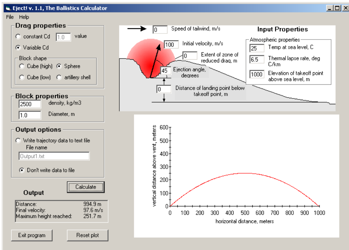
Figure 6. Graphical user interface for the program Eject!
